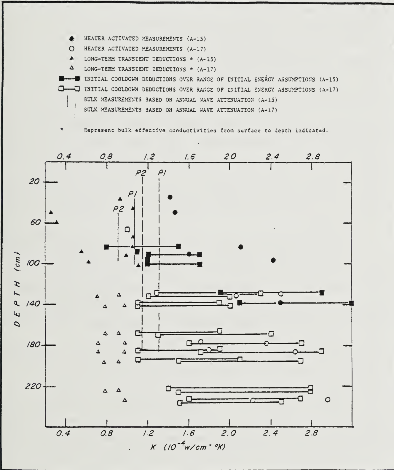
Conductivity deductions based on both short-term experiments and analyses of the long-time data
